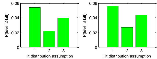
Figure 13: Probability kill values ( P_{KH} ) for survivability level 2 and 3 for the ship configuration 1 as a result of an RPG hit.
