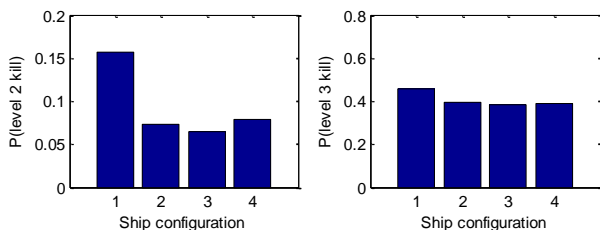
Figure 7: Probability kill values ( P_{KIH} ) for survivability level 2 and 3 a result of a 12.7mm machinegun salvo.
