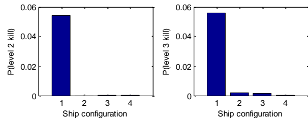
Figure 9: Probability kill values ( P_{KIH} ) for survivability level 2 and 3 a result of a RPG hit.
