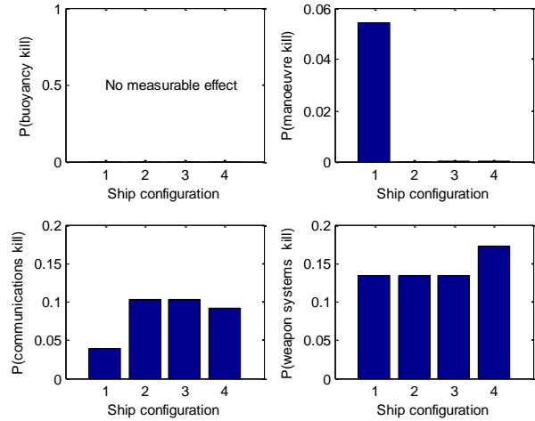
Figure 8: Probability values ( P_{KIH} ) for buoyancy kill manoeuvre kill, communication kill and weapon system kill for the four ship configurations as a result of a RPG hit. No measurable effect means that all probabilities are below 0.01.
