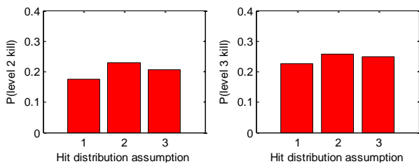
Figure 11: Probability kill values ( P_{KH} ) for survivability level 2 and 3 for the ship configuration 4 as a result of an ASM hit.
