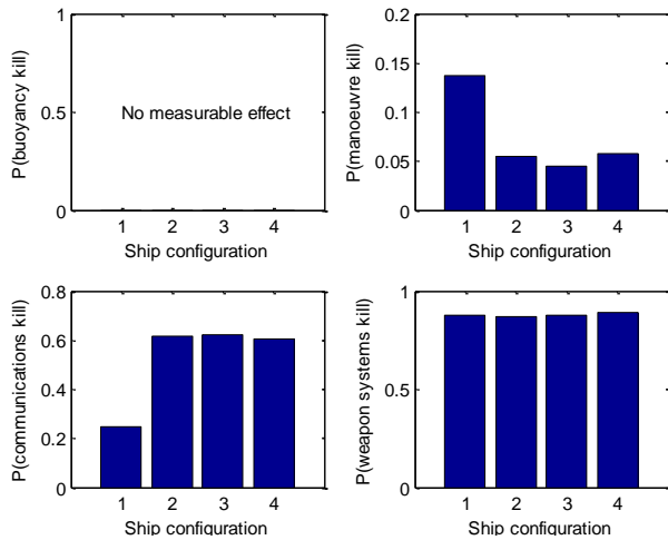
Figure 6: Probability values ( P_{KIH} ) for buoyancy kill manoeuvre kill, communication kill and weapon system kill for the four ship configurations as a result of a 12.7 mm machine gun salvo. No measurable effect means that all probabilities are below 0.01.
