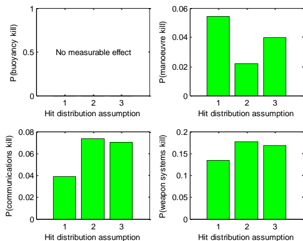
Figure 11: Probability kill values ( P_{KH} ) for survivability level 2 and 3 for the ship configuration 4 as a result of an ASM hit.
