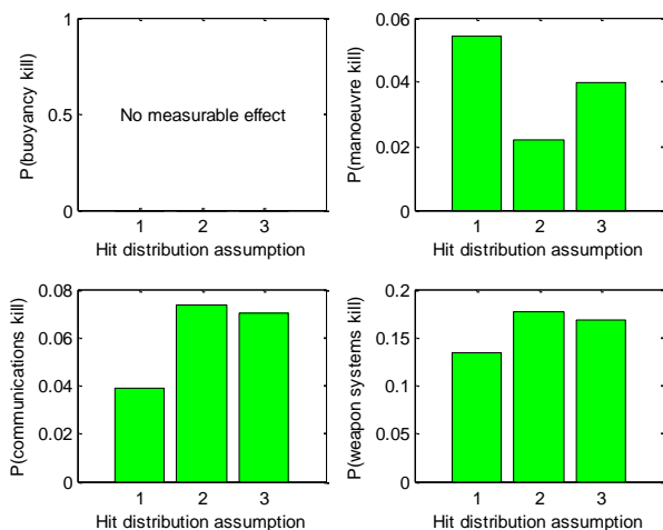
Figure 11: Probability kill values ( P_{KH} ) for survivability level 2 and 3 for the ship configuration 4 as a result of an ASM hit.
